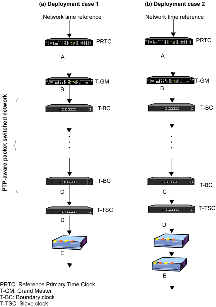
Figure 1.2 ITU-T G.8271.1 / G.8275.1 network reference model. The PTP endpoints are T-GMs and T-TSCs. All packet transmission / switching network elements implement the T-BC function.
