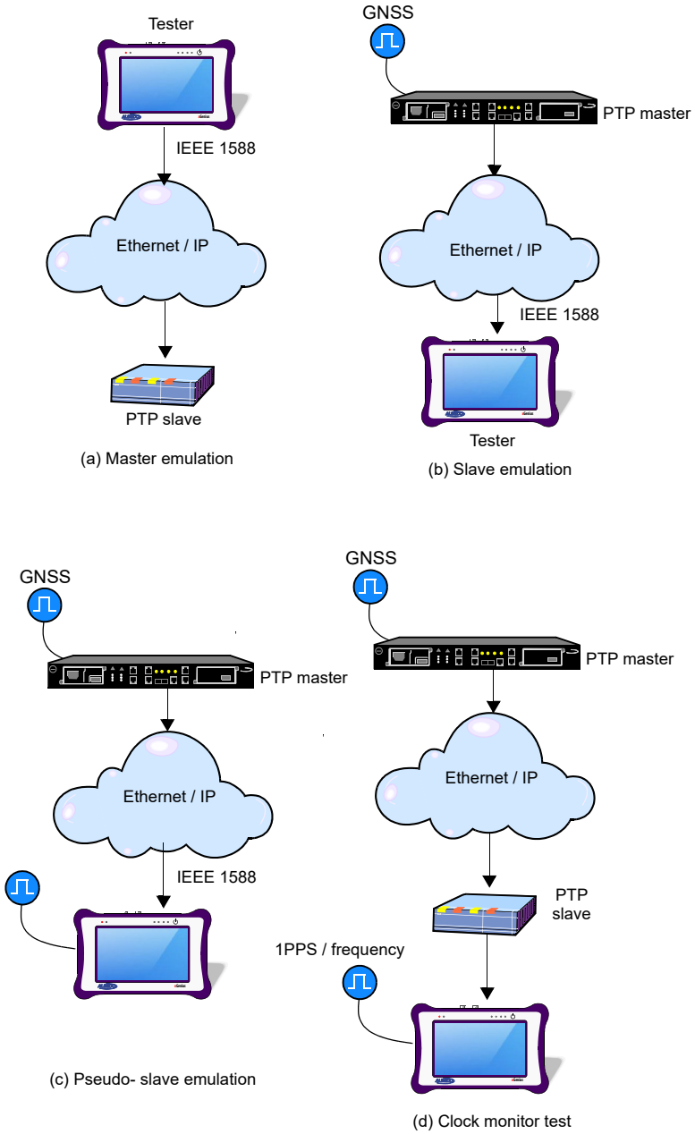
Figure 3.1 Basic PTP testing scenarios in endpoint mode: (a) Master emulation mode, (b) Slave emulation mode, (c) Pseudo-slave emulation mode, (d) Clock monitor mode
