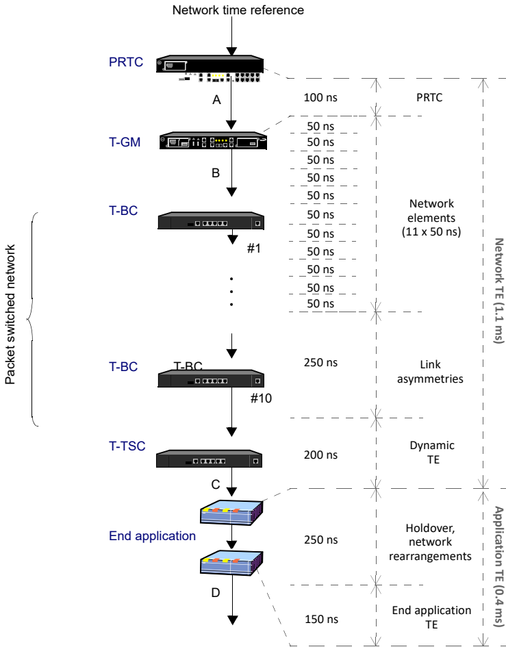
Figure 4.1 Time Error budget in a phase / time delivery application. TE control requires careful planning in these applications.
