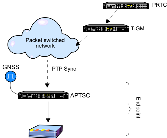
Figure 1.4 Comparison between the legacy distributed PRTC and APTS architectures.
