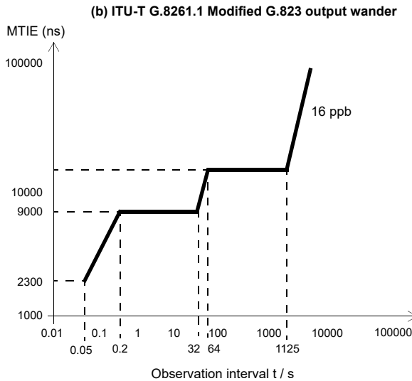
Figure 3.8 (a) ITU-T G.8261 EEC output wander option 1. Applies to the output of an EEC-1 b also may apply to a PEC-M and PEC-S. (b) ITU-T G.8261.1 modified ITU-T G.823 mask that applies to PEC-S output.
