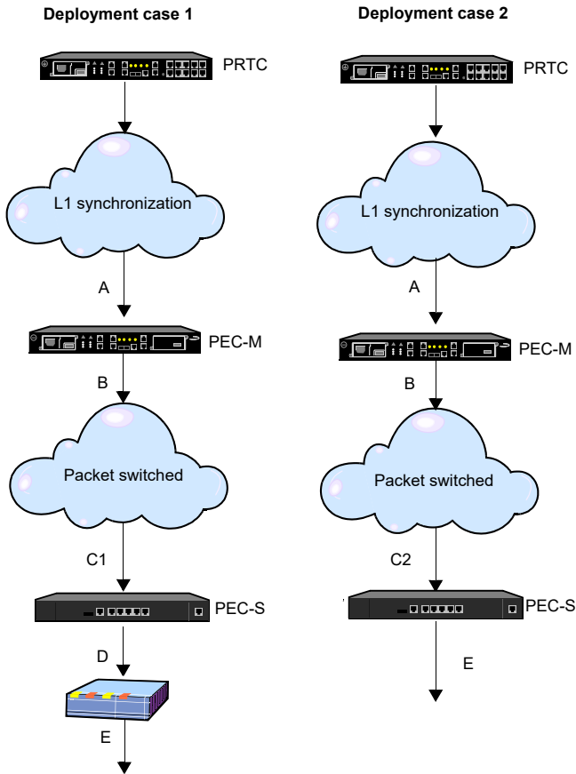
Figure 3.7 (ITU-T G.8261.1 reference model for frequency distribution applications. It includes both L1 synchronization and packet-based synchronization.
