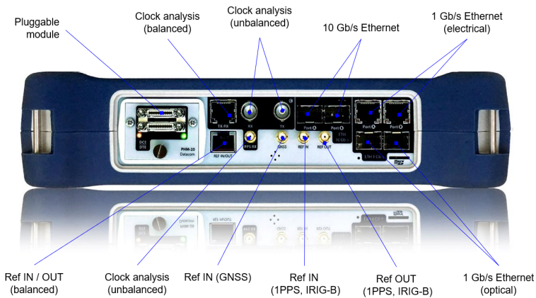
Figure 3.2 xGenius Test / Reference Port Panel
