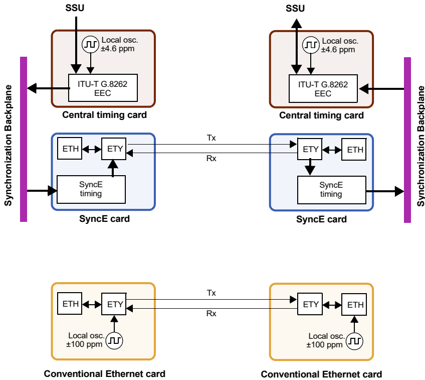
Figure 3.5 Synchronous Ethernet Architecture and comparison with conventional Ethernet
