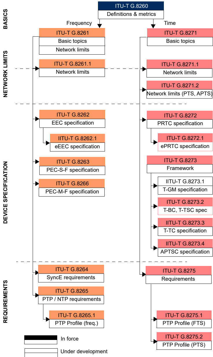
Figure 1.1 ITU-T packet switched network timing and synchronization standards.
