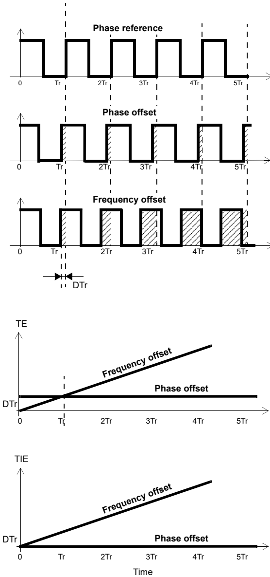
Figure 2.4 Differences between TE and TIE. The TE is the difference between two times and the TIE is the difference between two time intervals
