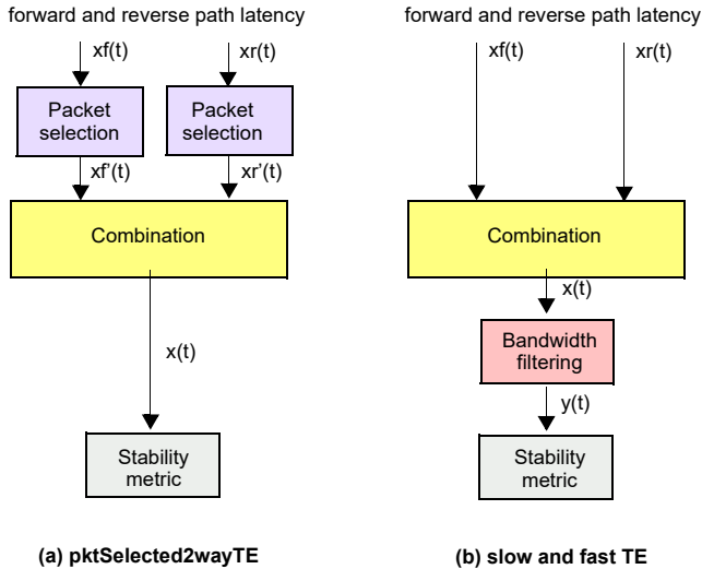
Figure 4.4 ITU-T G.8260 metrics derived from the raw TE: (a) pktSelected2wayTE , (b) slow and fast TE . The bandwidth filter is a 0.1 Hz low-pass filter for the slow TE and a 0.1 Hz high-pass filter for the fast TE
