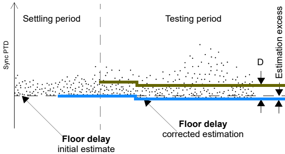
Figure 3.10 Illustration of the floor delay population test. Samples are classified as conforming or not conforming depending on the latency the experience from the grandmaster computed from the floor delay.
