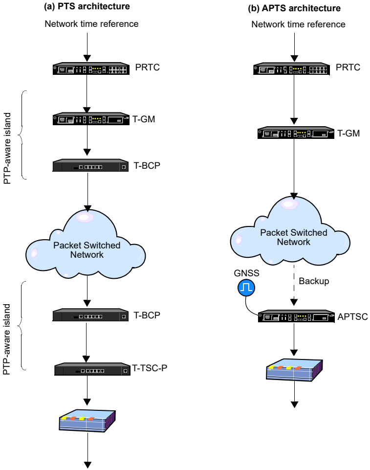
Figure 1.3 Architectures considered in ITU-T G.8275 and ITU-T G.8275.2 for time and phase distribution through networks with partial timing support.
