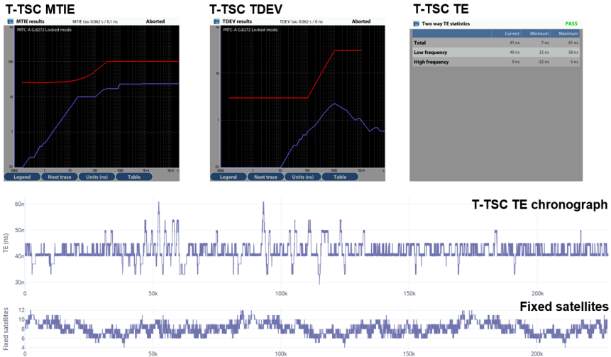
Figure 3.4 Basic PTP analysis with xGenius
