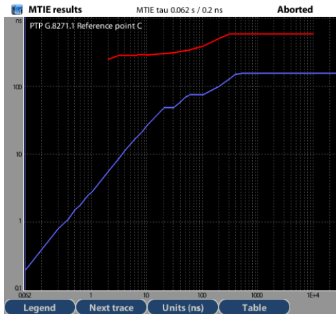
Figure 3.6 MTIE Results with xGenius.
