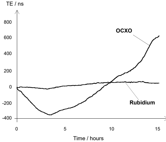
Figure 2.6 Rubidium and OCXO holdover performances in a 15hour TE test. Both tests have been run at the output of a PRTC. Environmental conditions were the same the OCXO and Rubidium devices but the Rubidium clock exhibits a much better performance.
