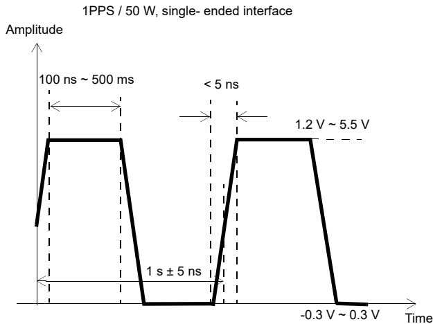
Figure 4.2 1PPS pulse shape specification in 50 \Omega , single ended interfaces. This interface is described in ITU-T G.703 and G.8271.
