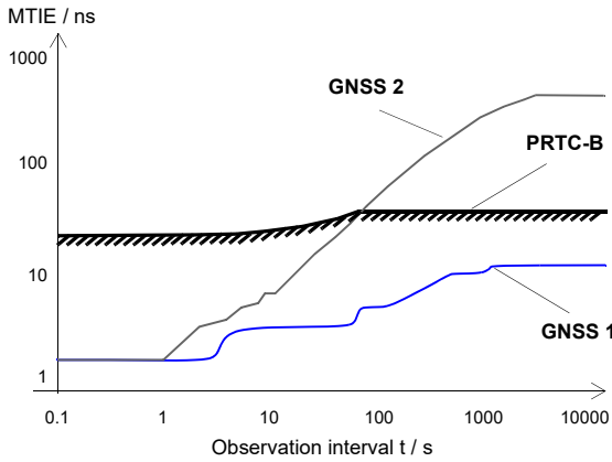
Figure 2.5 The same MTIE measurement carried over with two different GNSS references (GNSS 1 and GNSS 2) and the same local oscillator (Rubidium). Using a bad reference may completely change the test results
