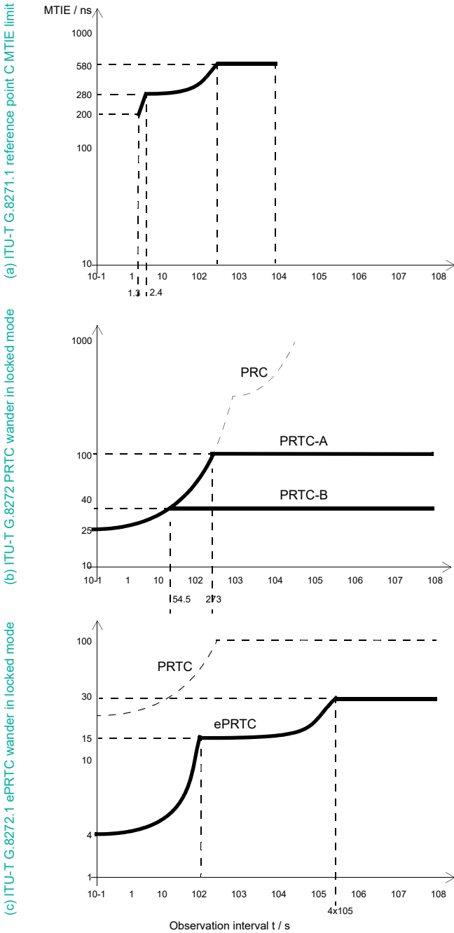
Figure 4.3 MTIE limits at the PRTC / ePRTC output and at the input of the T-TSC in a phase / time delivery application.
