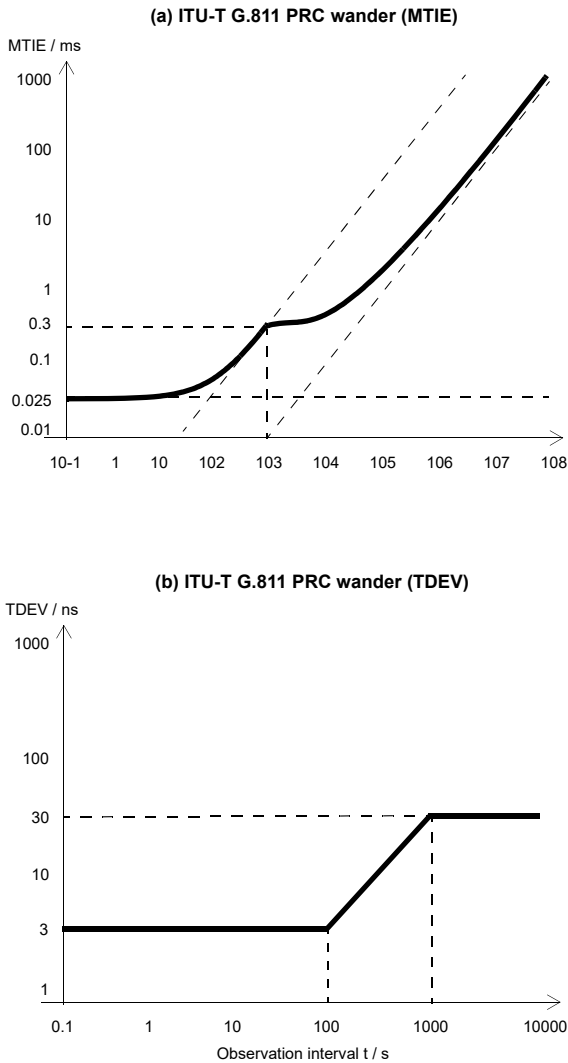
Figure 2.3 ITU-T G.811 performance limits of a PRC expressed in terms of MTIE and TDEV.
