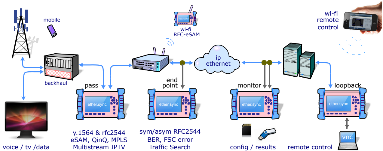
Figure 2 ALBEDO Ether.Genius / Ether.Sync / Ether.Giga field testers in operation.
